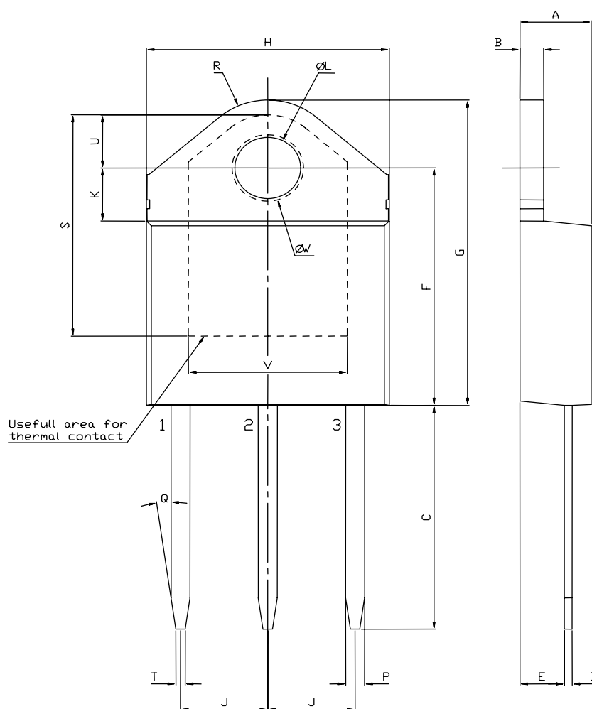
Figure 8. Package outline
