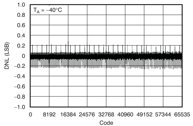
Figure 9. Differential Nonlinearity vs Digital Input Code
