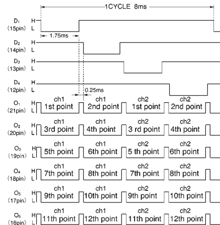
Timing chart for all LEDs on (f = 4kHz)
