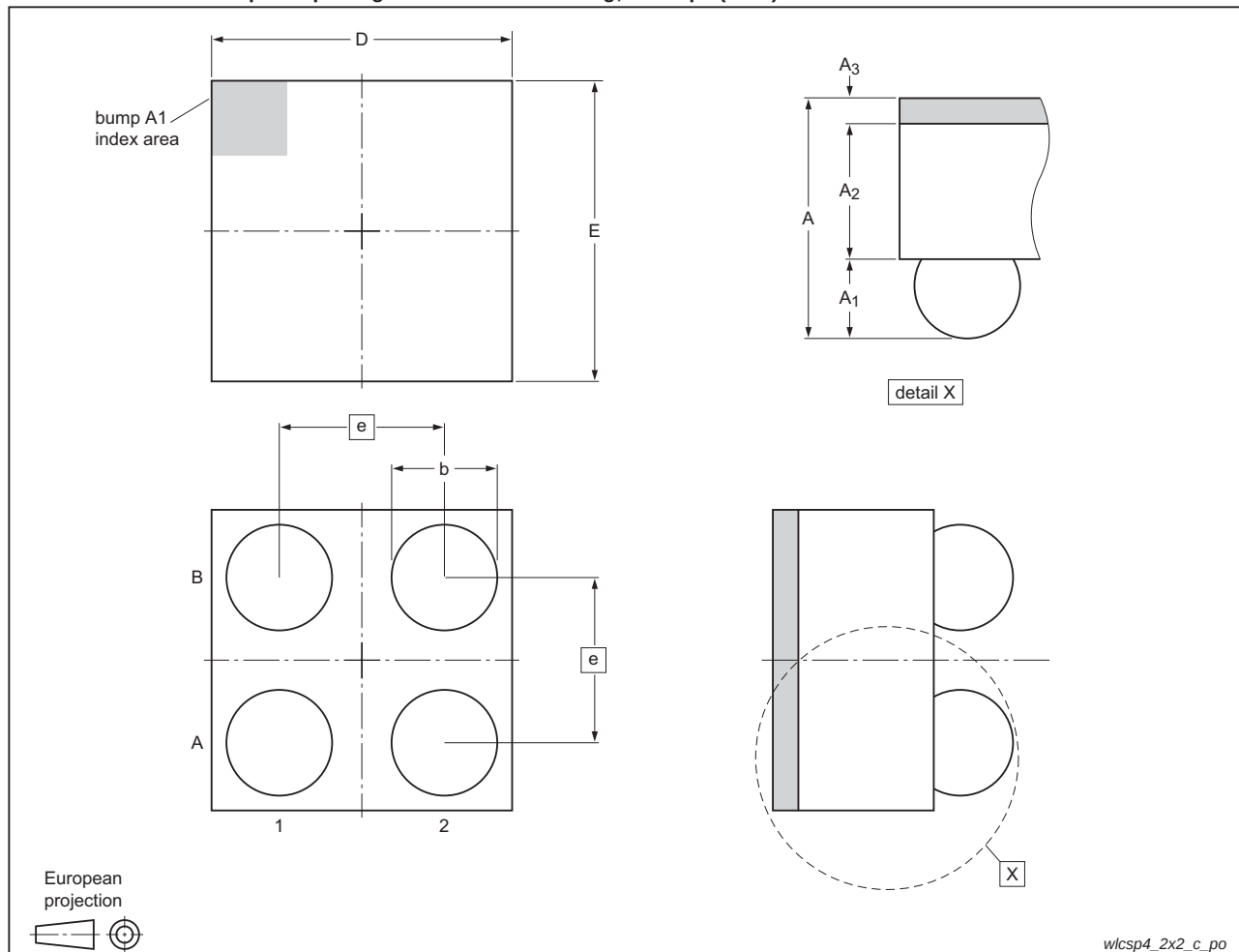
WLCSP4: wafer level chip-size package with backside coating; 4 bumps (2 x 2)
