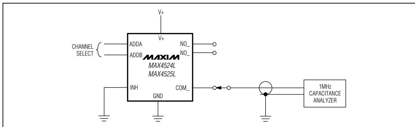
Figure 5. NO/COM Capacitance
