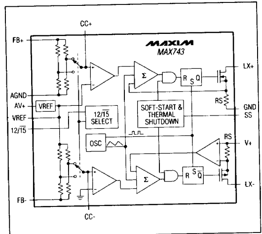
Figure 3. MAX743 Block Diagram
