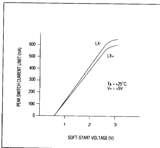
Figure 10. Typical Peak Switch Current Limit vs. Soft-Start Voltage
