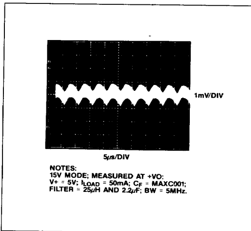
Figure 9. Output Noise Voltage with Pi Filter
