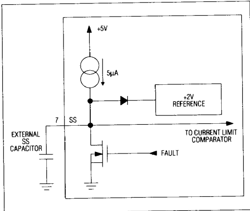
Figure 11. Soft-Start Equivalent Circuit
