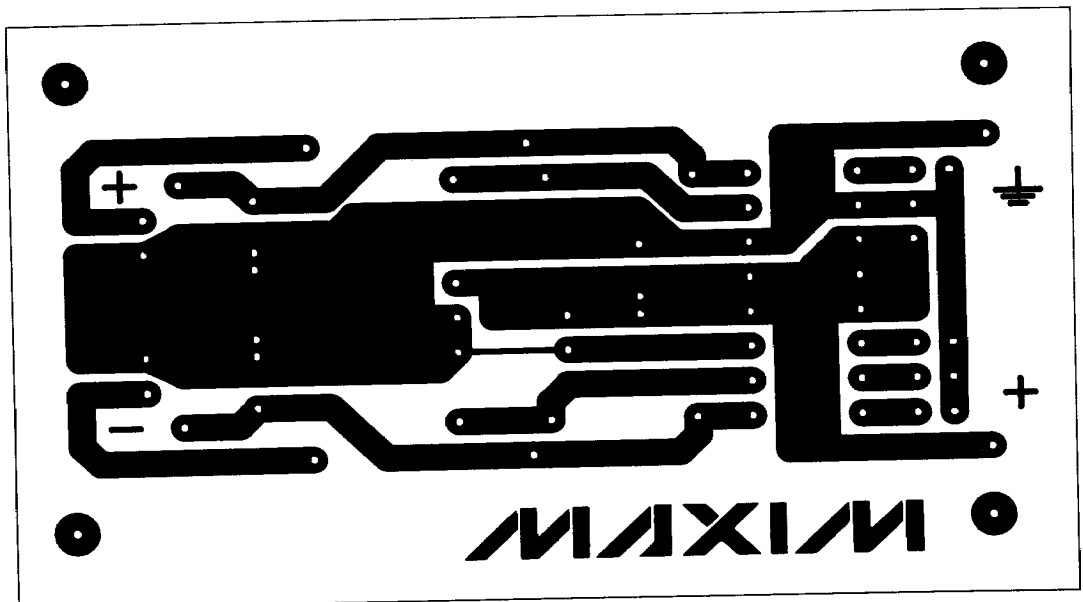
Figure 6. PC Layout for Circuit of Figure 4 Using MAXL001/MAXC001 (2X Scale)
