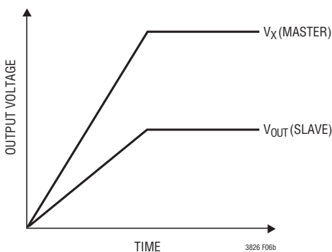
Figure 6. Two Different Modes of Output Voltage Tracking
