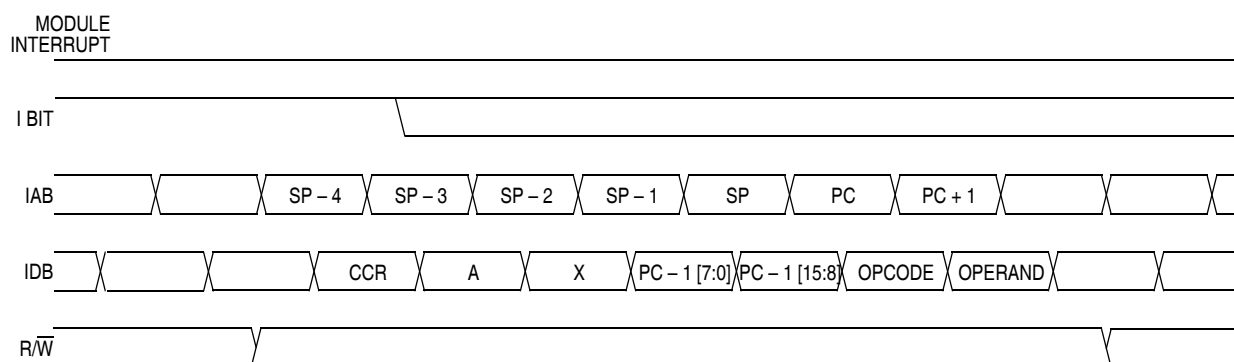
Figure 14-8. Interrupt Recovery
