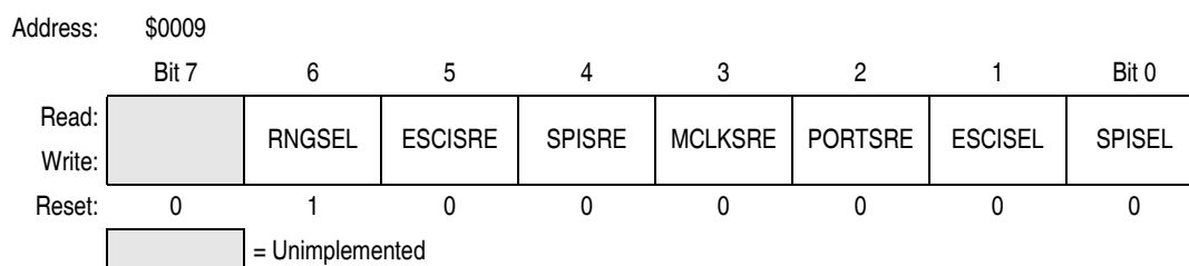
Figure 5-3. Configuration Register 3 (CONFIG3)
