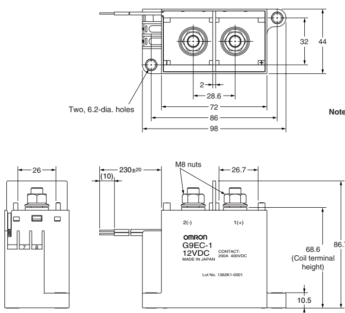
Mounting Hole Dimensions (TOP VIEW)
