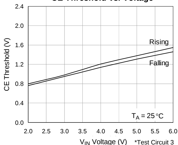
CE Threshold vs. Voltage
