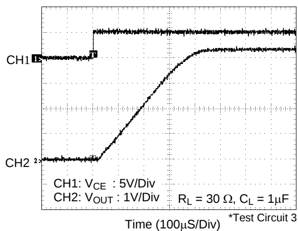
Turn-On Response
