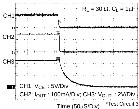
Turn-Off Response
