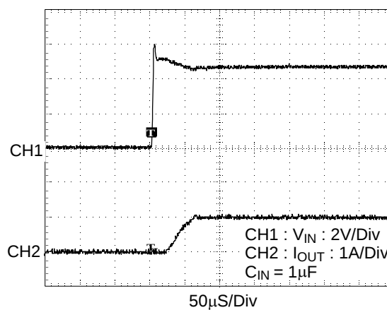
Soft-start Short Circuit Response
