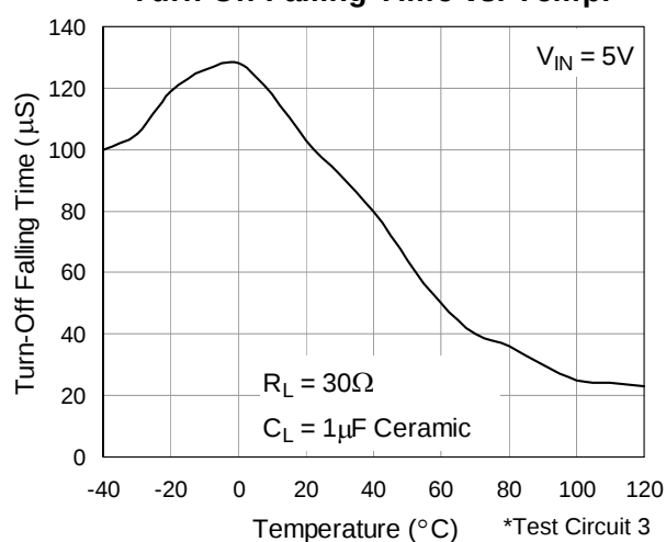
Turn Off Falling Time vs. Temp.
