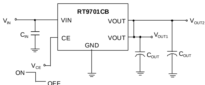
Fig. 2 High Side Power Switch with Chip Enable Control
