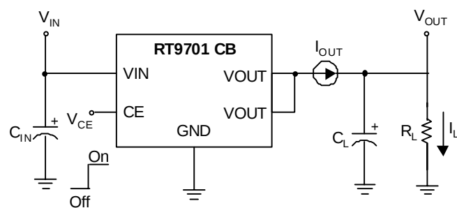
Test Circuit 3
