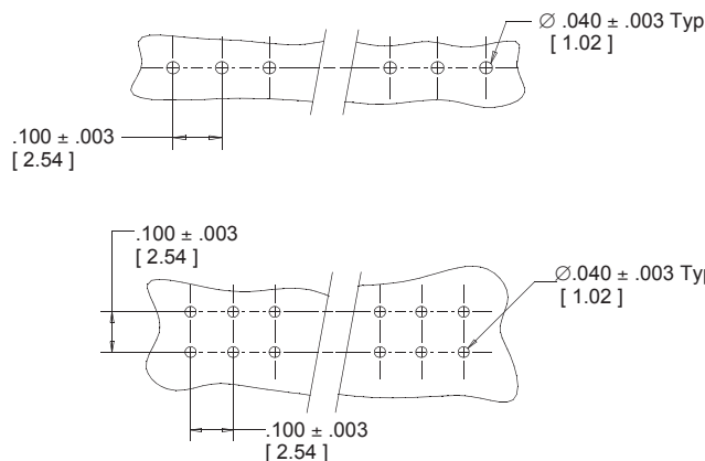
Recommended Mounting Hole Patterns (Shown for Mounting Side of Board)
