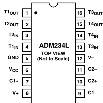
Figure 9. ADM234L DIP/SOIC Pin Configuration
