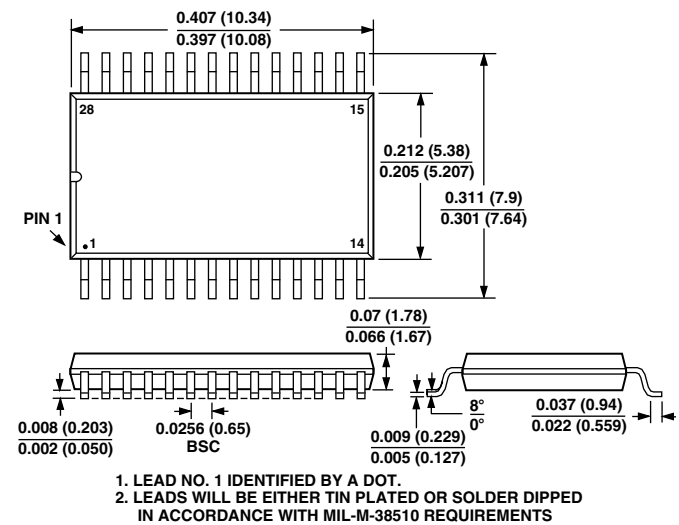
28-Lead SSOP (RS-28)
