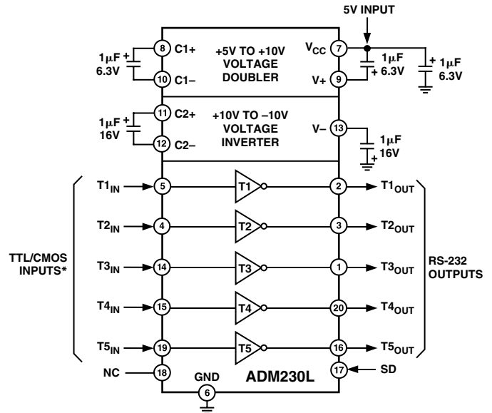
* INTERNAL 400kΩ PULL-UP RESISTOR ON EACH TTL/CMOS INPUT.
