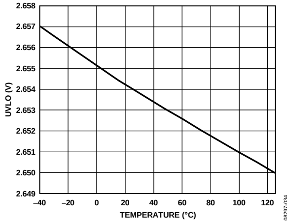
Figure 34. UVLO vs. Temperature
