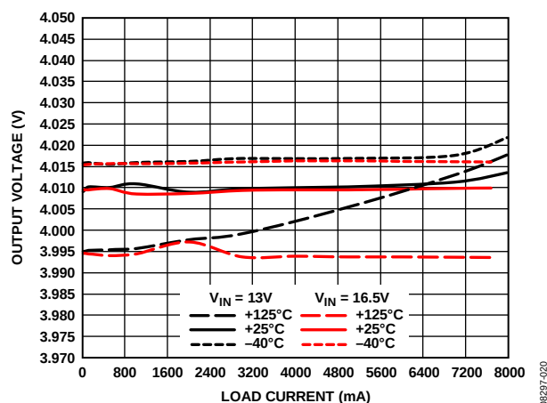
Figure 20. Output Voltage Accuracy—1.0 MHz, V_{OUT} = 4 V
