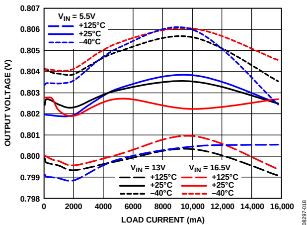
Figure 18. Output Voltage Accuracy—1 MHz, V_{OUT} = 0.8 V
