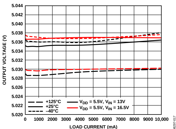
Figure 17. Output Voltage Accuracy—600 kHz, V_{OUT} = 5 V
