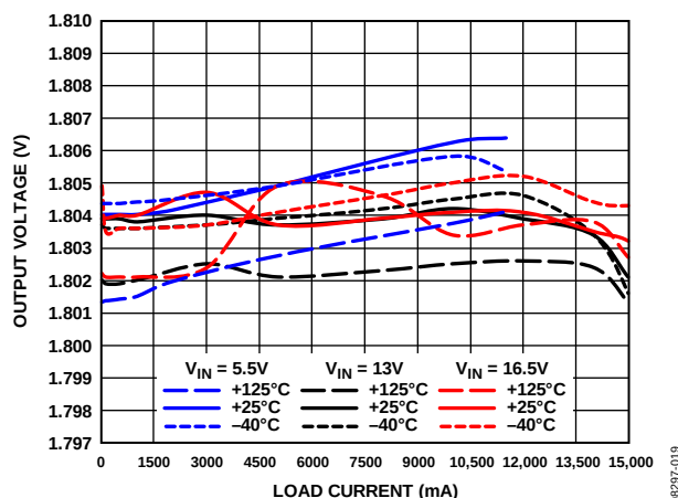
Figure 19. Output Voltage Accuracy—1.0 MHz, V_{OUT} = 1.8 V
