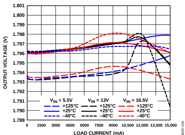
Figure 16. Output Voltage Accuracy—600 kHz, V_{OUT} = 1.8 V
