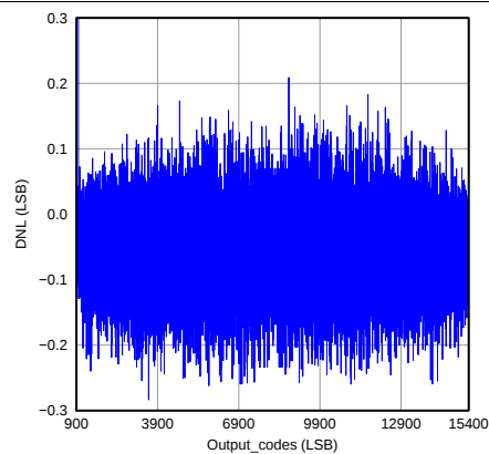
Figure 27. Differential Non-Linearity
