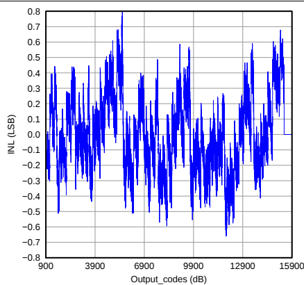
Figure 26. Integral Non-Linearity
