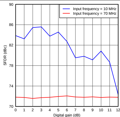
Figure 17. SFDR vs Digital Gain
