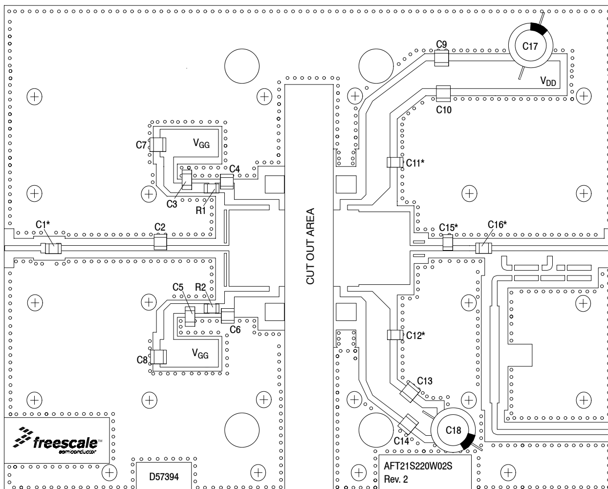
Figure 2. AFT21S220W02SR3 Test Circuit Component Layout
