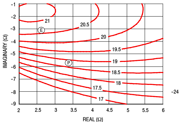
Figure 10. P1dB Load Pull Gain Contours (dB)
