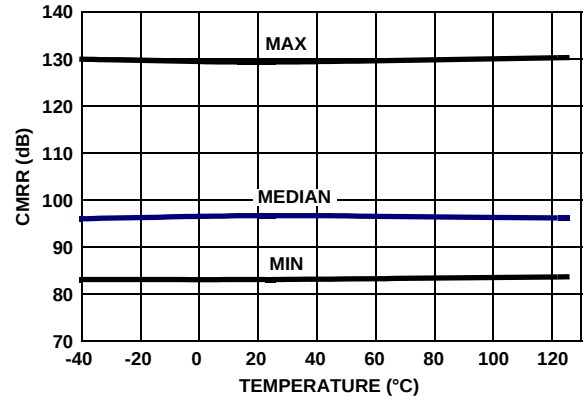
FIGURE 31. CMRR vs TEMPERATURE V_{CM} = -2.5V TO +2.5V , V_+ , V_- = \pm 2.5V
