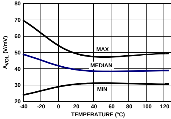
FIGURE 30. A_{VOL} vs TEMPERATURE R_L = 1k , V_+ , V_- = \pm 2.5V , V_O = -2V TO +2V
