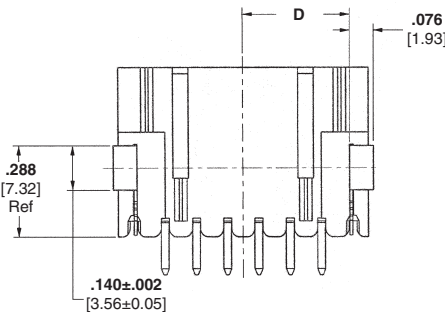
Section K-K
