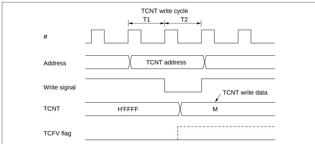
Figure 9-53 Contention between TCNT Write and Overflow
