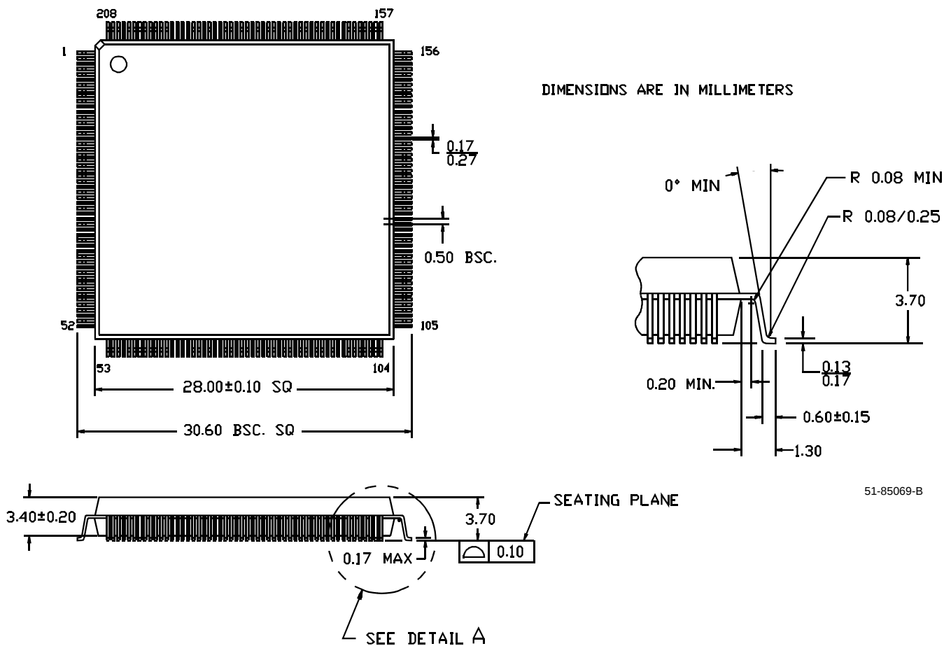
208-Lead Plastic Quad Flatpack (EQFP) NT208
