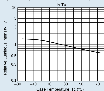
Example: Temperature dependence of optical output
