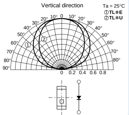
Radiation pattern
