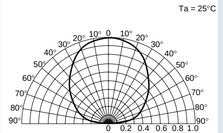
Radiation pattern
