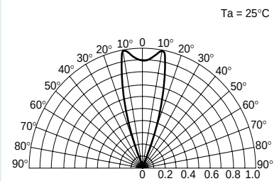
Radiation pattern
