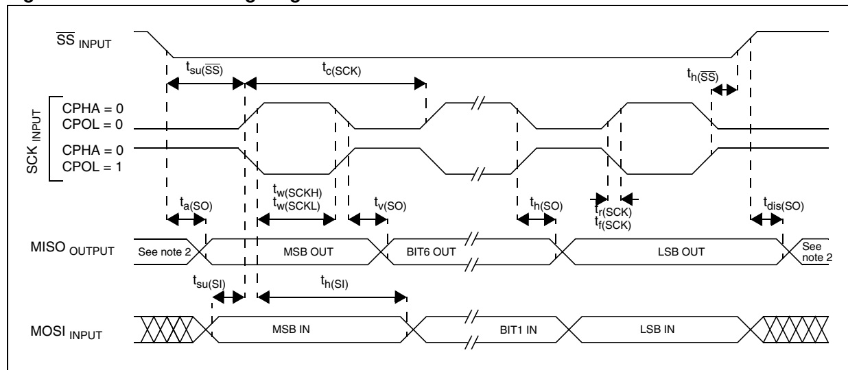
Figure 138. SPI Slave Timing Diagram with CPHA = 0^{(3)}
