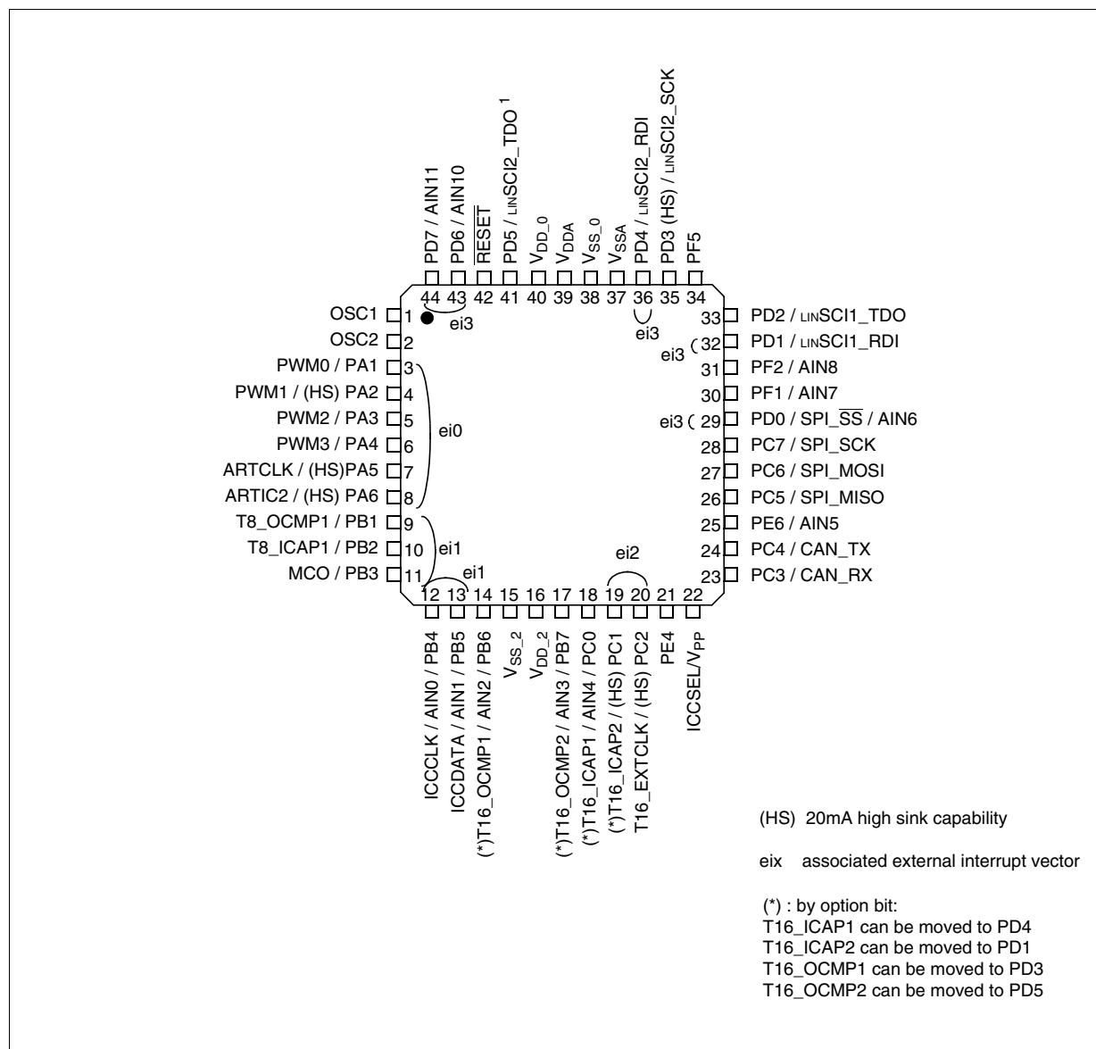
Figure 3. LQFP 44-Pin Package Pinout
