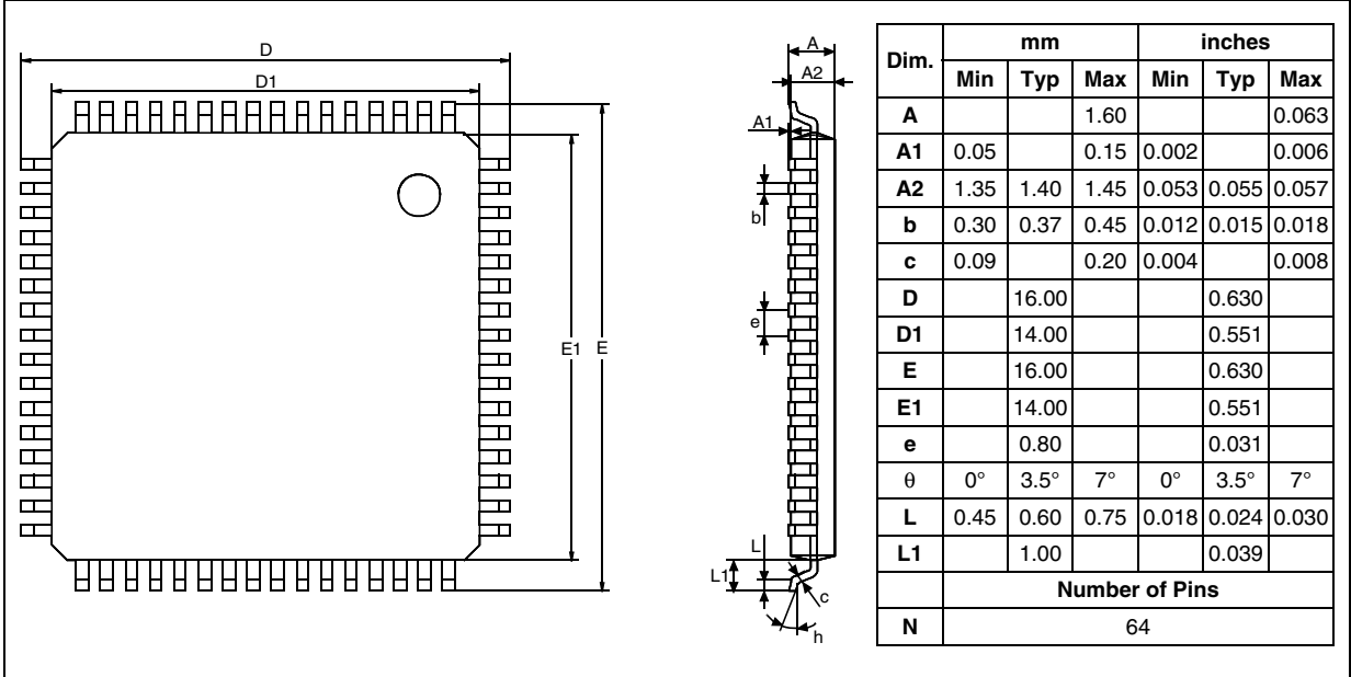
Figure 146. 64-Pin Low Profile Quad Flat Package (14x14)
