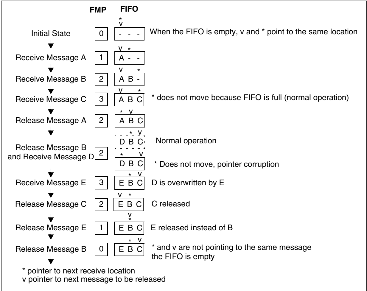
Figure 109. FIFO Corruption
