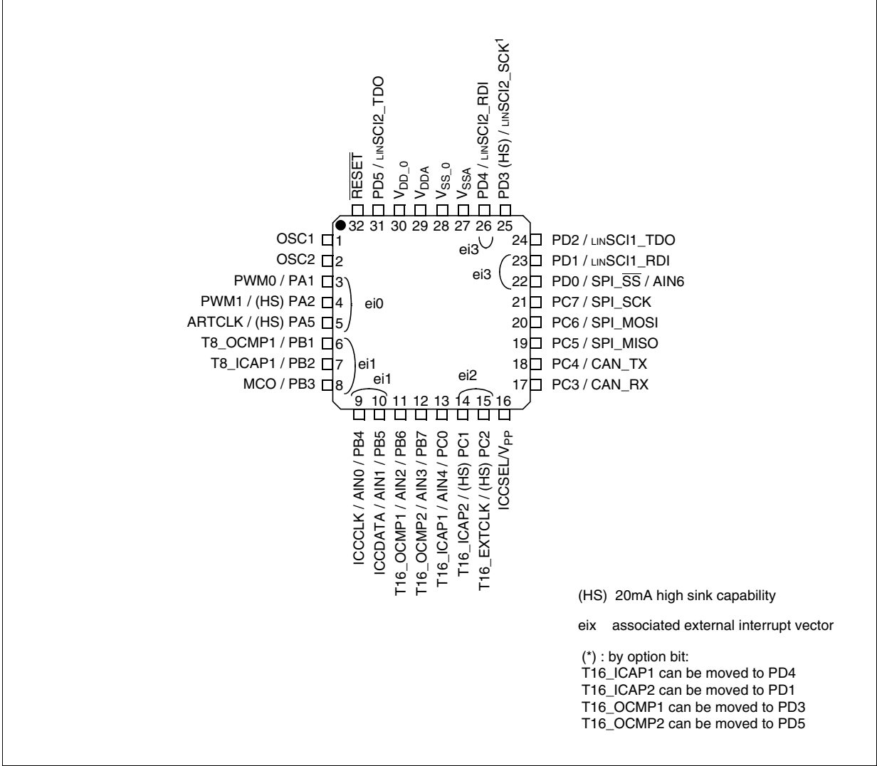
Figure 4. LQFP 32-Pin Package Pinout
