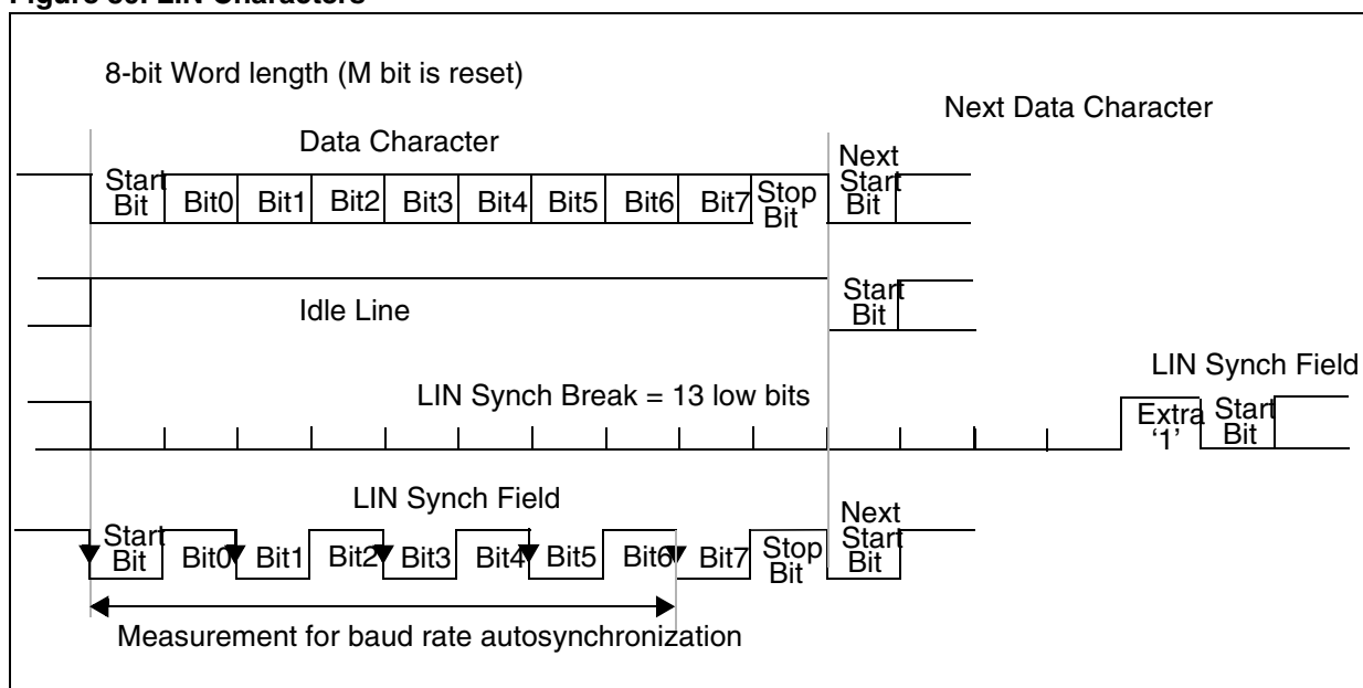
Figure 80. LIN Characters
