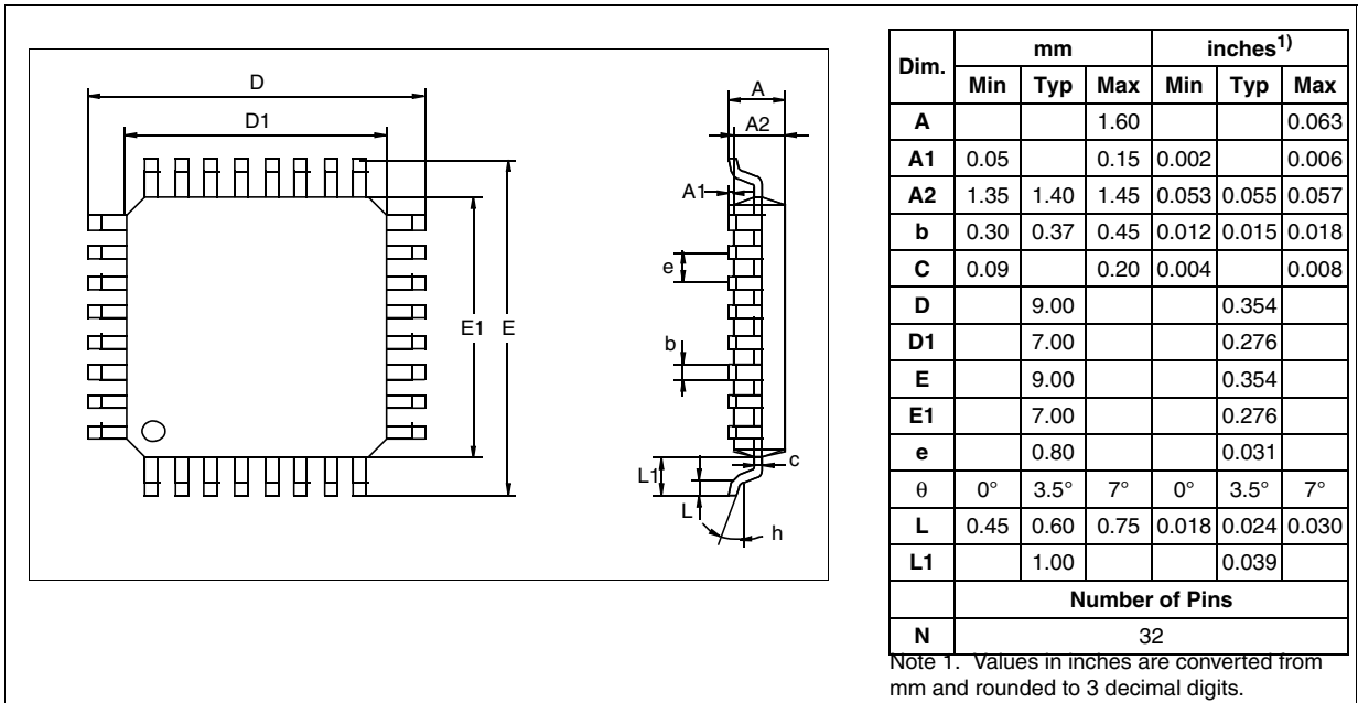
Figure 147. 32-Pin Low Profile Quad Flat Package (7x7)
