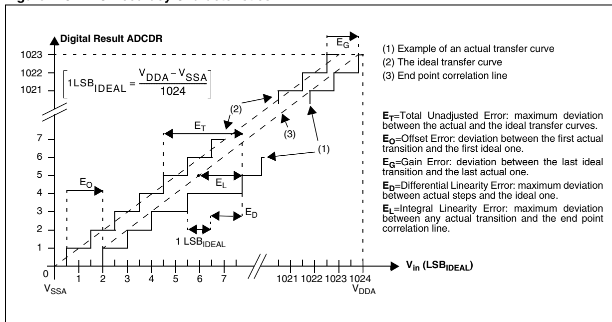
Figure 145. ADC Accuracy Characteristics
