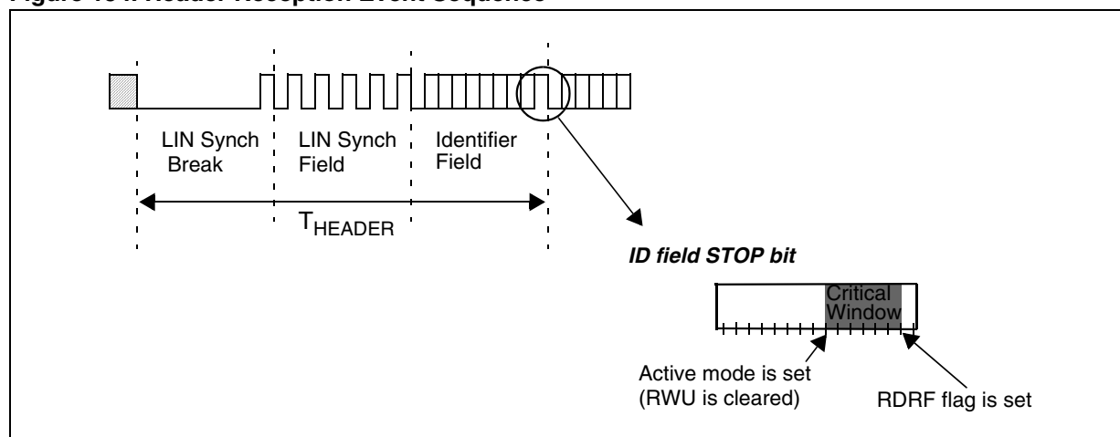
Figure 154. Header Reception Event Sequence
