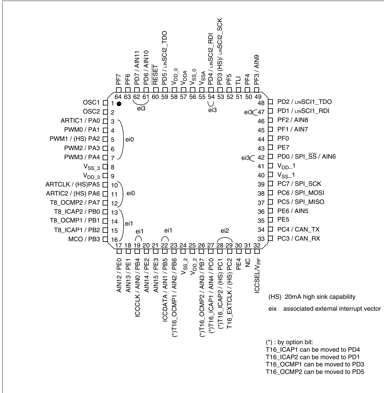
Figure 2. LQFP 64-Pin Package Pinout
