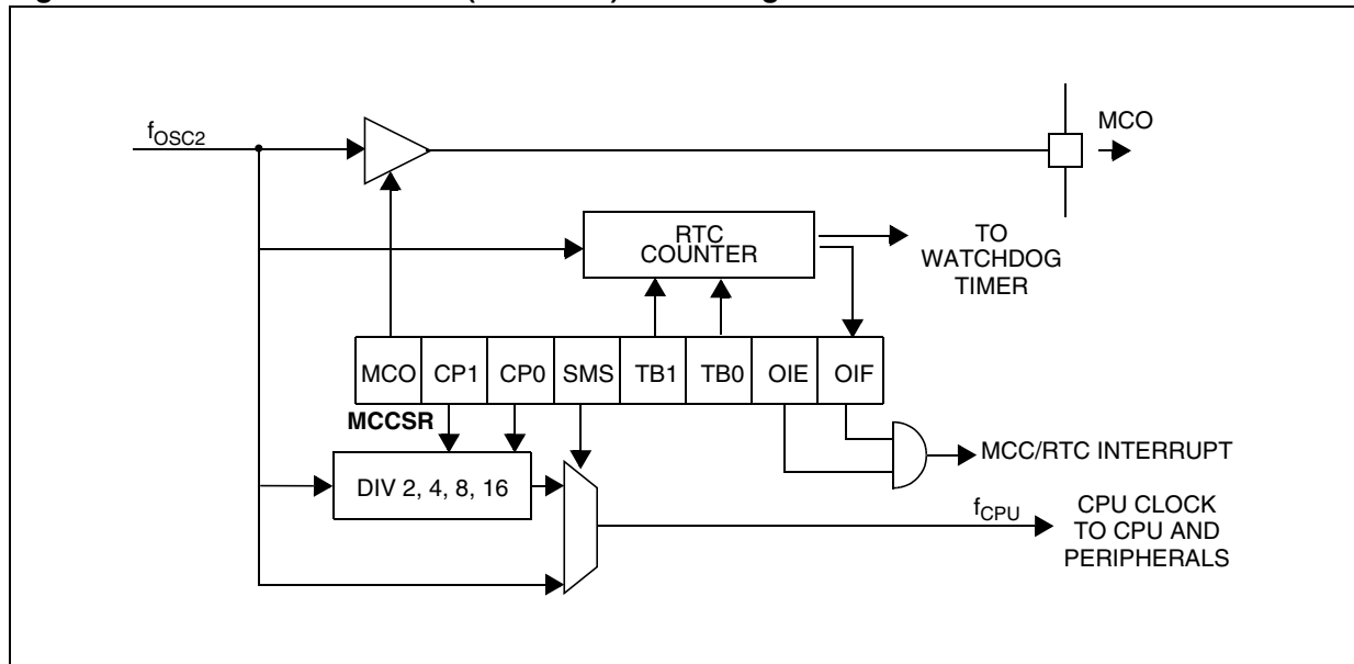
Figure 39. Main Clock Controller (MCC/RTC) Block Diagram
