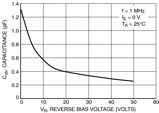
Figure 45. Output Capacitance
