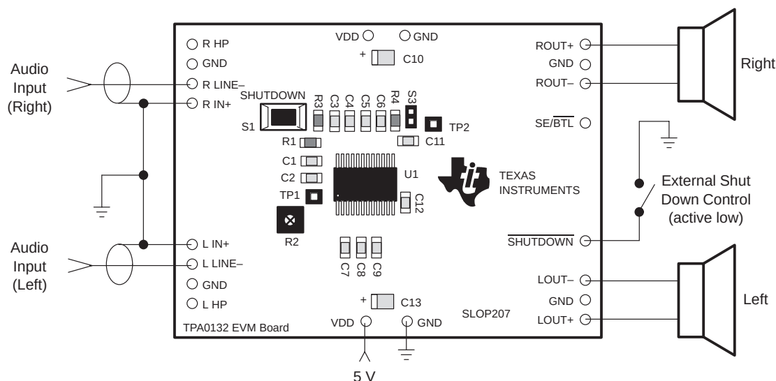
Figure 3–9. TPA0132 EVM Connected for Stereo BTL Output
