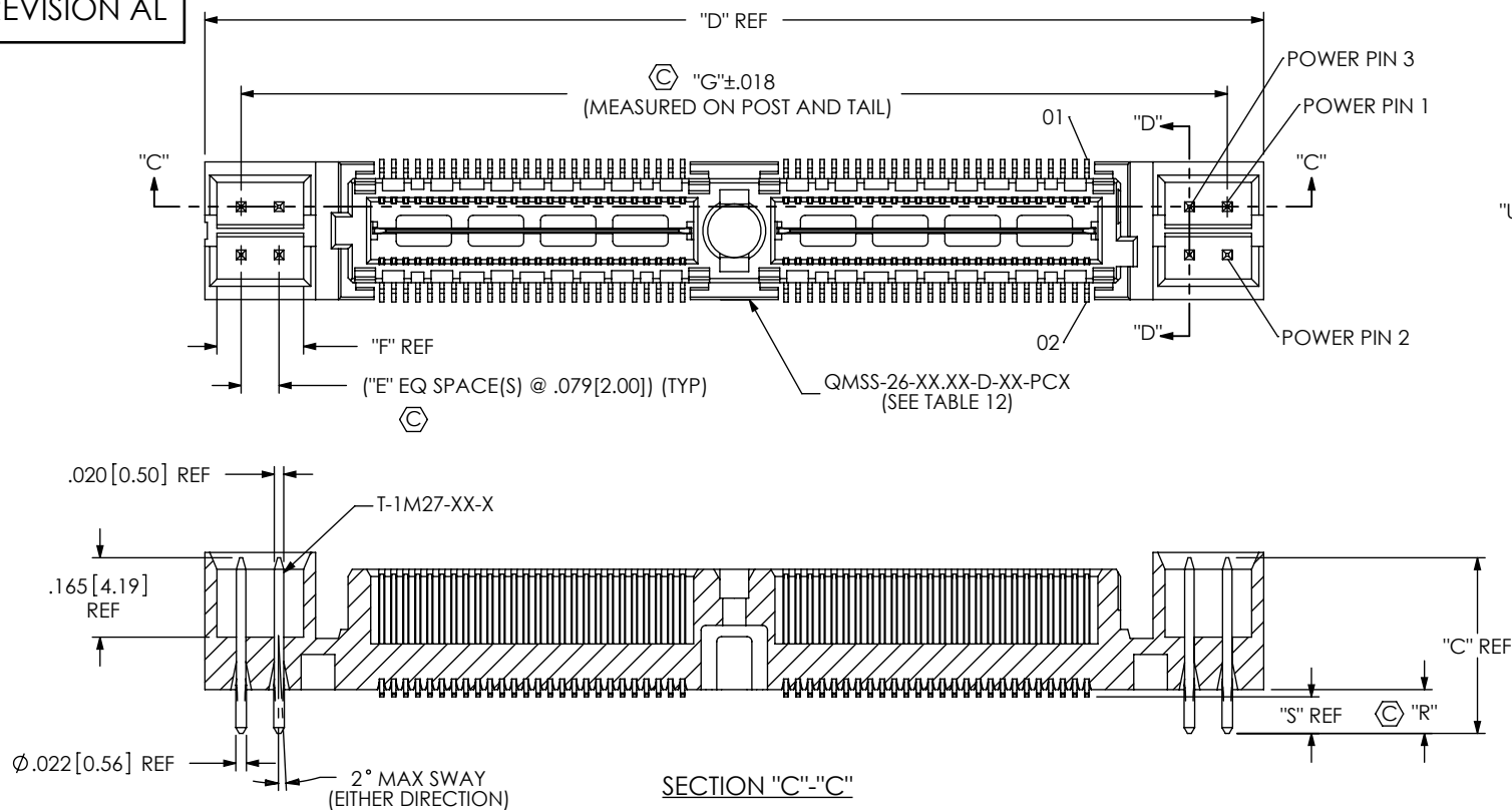
FIG 5 -PXX OPTION POWER COMBO OPTIONS QMS-052-06.75-X-D-PC4 SHOWN (SAME AS FIG 1, UNLESS OTHERWISE STATED) [NOT AVAILABLE WITH -A, -GP OR -K OPTION, AVAILABLE ON LEAD STYLES -05.75 & -06.75 ONLY] (AVAILABLE ON -026, -052 & -078 POSITIONS ONLY)
