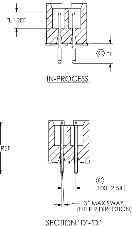
FIG 5 -PXX OPTION POWER COMBO OPTIONS QMS-052-06.75-X-D-PC4 SHOWN (SAME AS FIG 1, UNLESS OTHERWISE STATED) [NOT AVAILABLE WITH -A, -GP OR -K OPTION, AVAILABLE ON LEAD STYLES -05.75 & -06.75 ONLY] (AVAILABLE ON -026, -052 & -078 POSITIONS ONLY)
