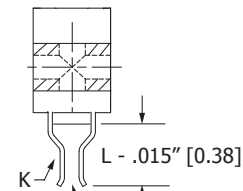
CARD EXTENDER REQUIRES -S288 MODIFICATION CODE (CS,CM,CT,RS,CK,TK,RM)
