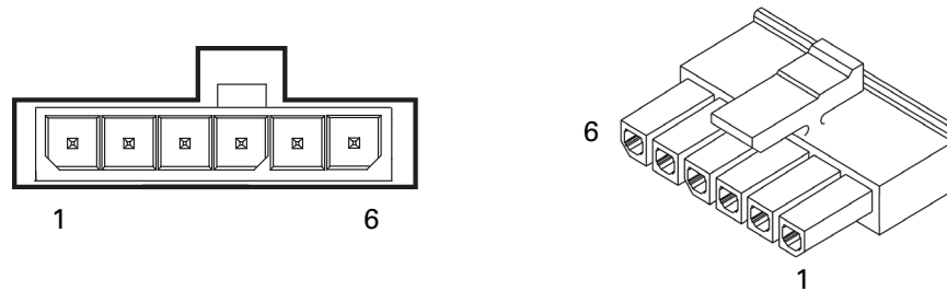
FIGURE 13. Hall Sensors connector
