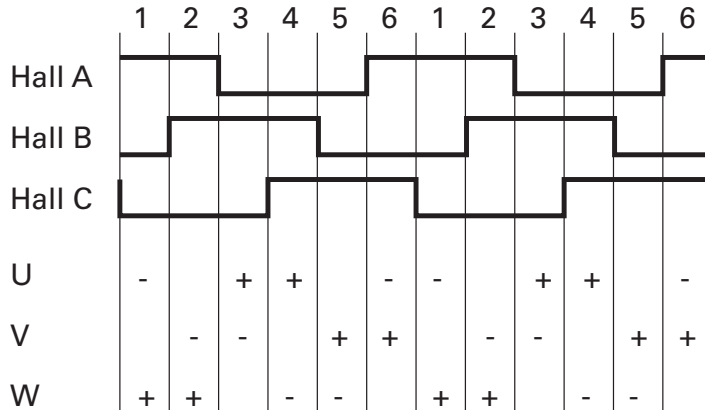
FIGURE 14. Hall Sensors sequence
