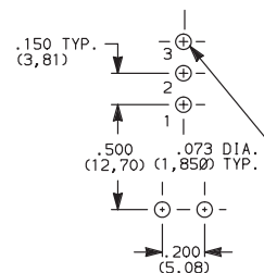
PC MOUNTING
