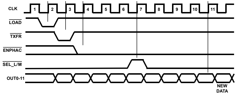
FIGURE 3. I/O TIMING
