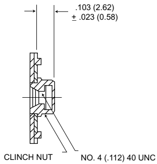
E-Clinch Nut
