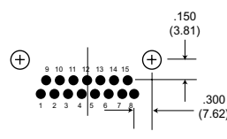
15 Contacts
