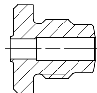
126303 DRIVING ANVIL -06
