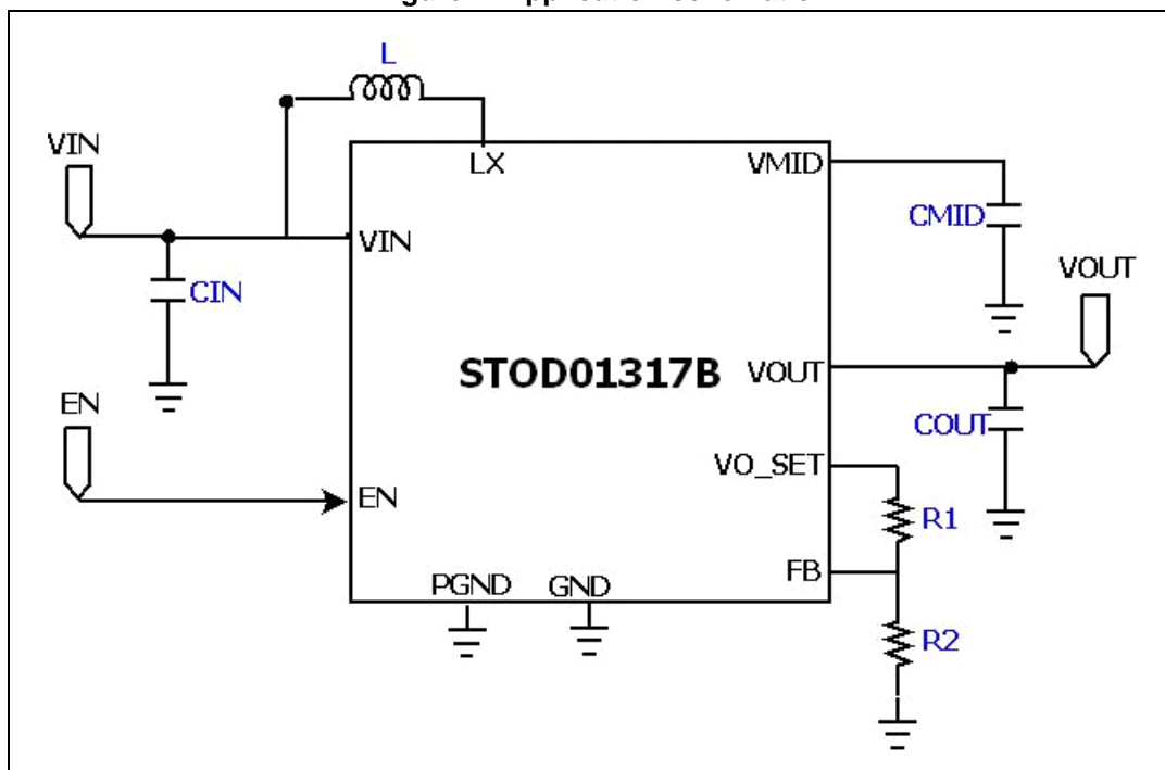
Figure 1. Application schematic
