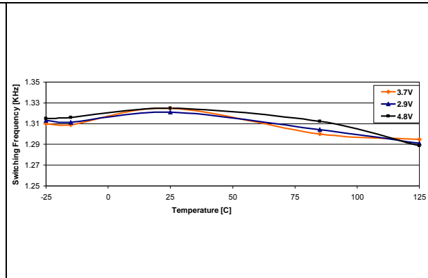
Figure 7. Switching frequency
