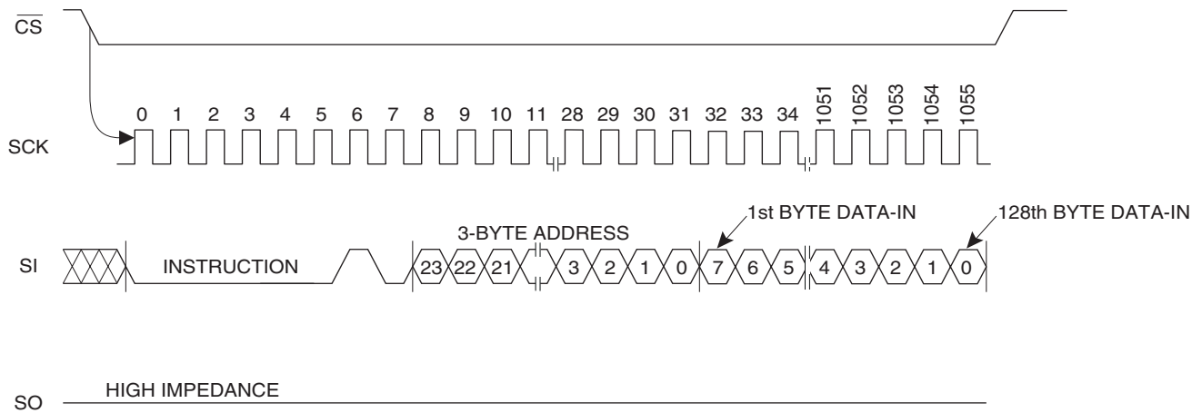
Figure 9. WRITE Timing
