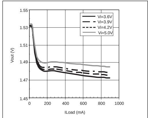
Figure 4. Line/Load Rejection, V_{OUT} = 1.5\text{V}
