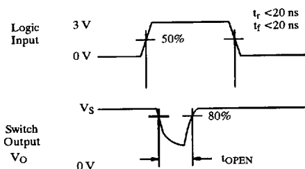
Figure 4. Break-Before-Make
