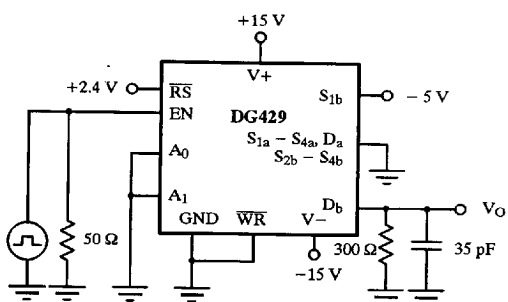
Figure 6. Enable t_{ON}/t_{OFF} Time
