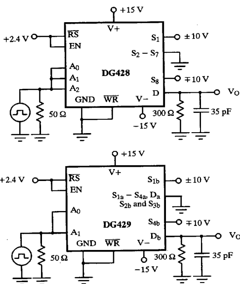
Figure 5. Transition Time
