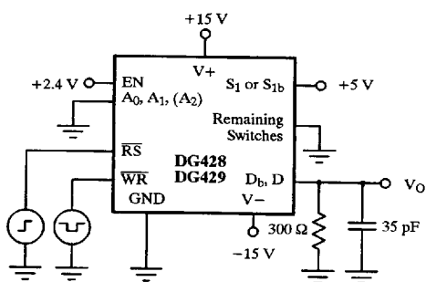
Figure 7. Write Turn-On Time t_{ON(WR)}
