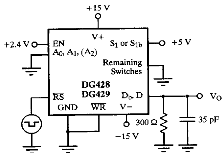
Figure 8. Reset Turn-Off Time t_{OFF}(RS)
