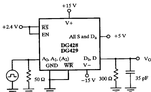
Figure 4. Break-Before-Make
