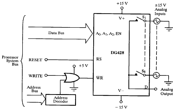
Figure 10. Bus Interface
