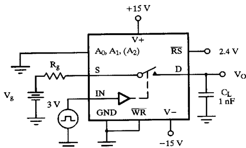
Figure 9. Charge Injection
