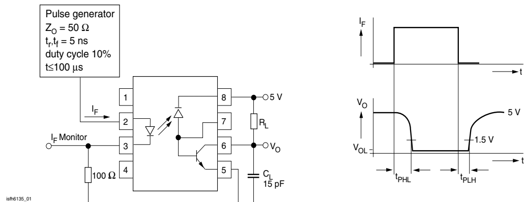
Figure 1. Schematics
