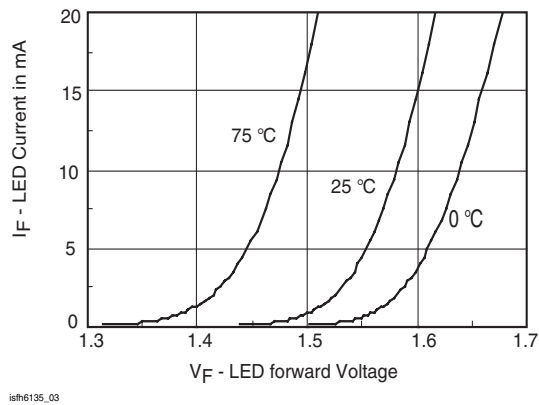
Figure 3. LED Forward Current vs. Forward Voltage
