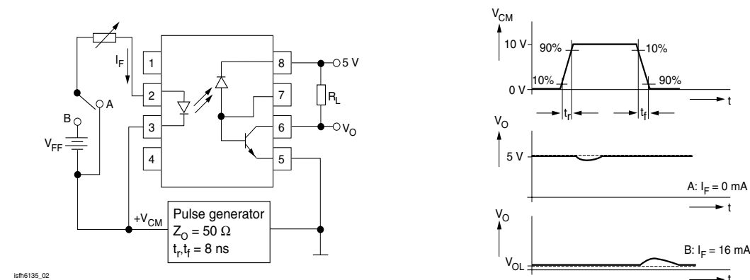
Figure 2. Common-Mode Interference Immunity
