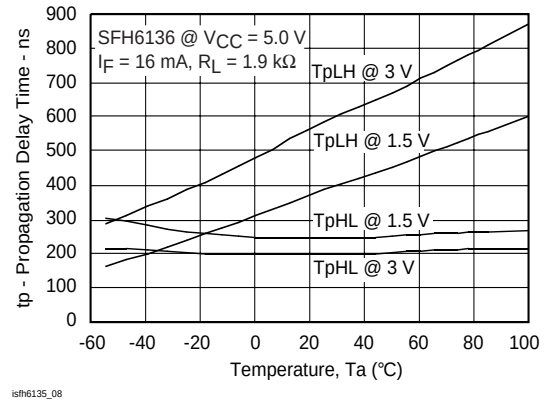
Figure 8. Propagation Delay vs. Temperature-SFH6136
