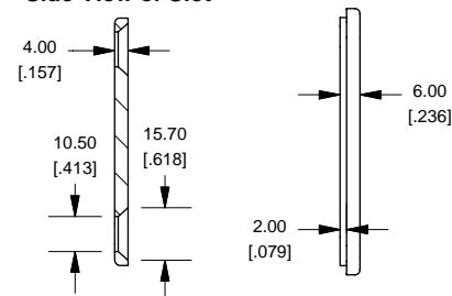
SECTION C-C Side View of Slot
