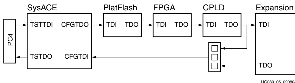
Figure 5: JTAG Chain
