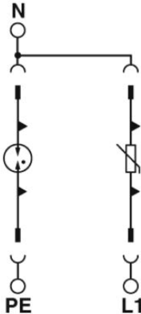
Circuit diagram
