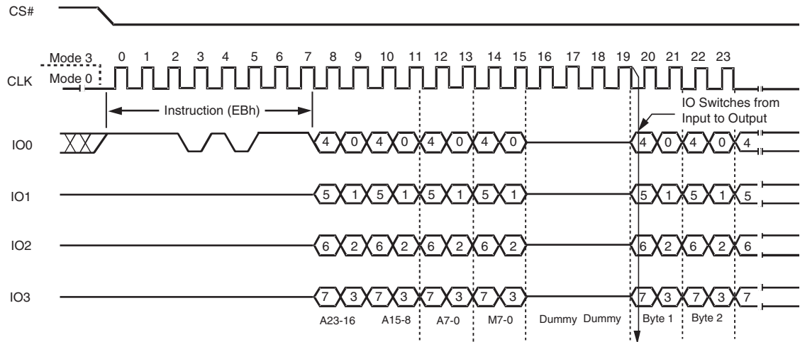
Figure 7.12 Fast Read Quad I/O Instruction Sequence (Initial instruction or previous M5-4 \neq 10)
