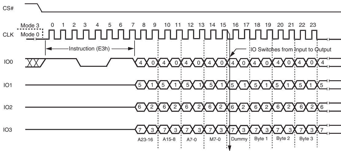
Figure 7.16 Octal Word Read Quad I/O Instruction Sequence (Initial instruction or previous M5-4 \neq 10)
