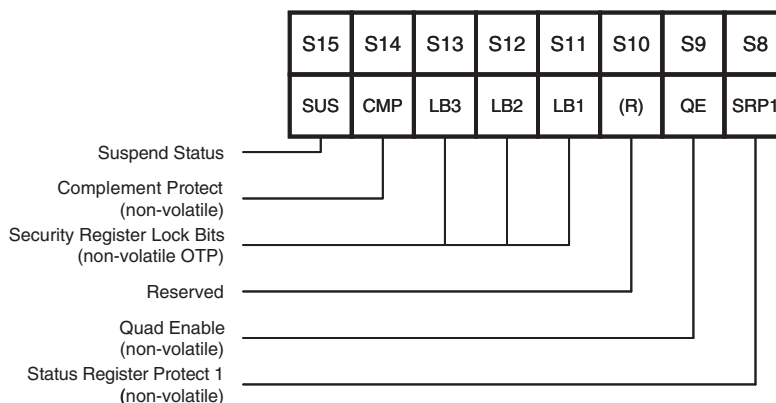
Figure 6.2 Status Register 2
