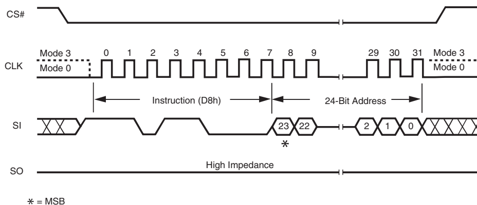
Figure 7.24 64 kB Block Erase Instruction Sequence Diagram
