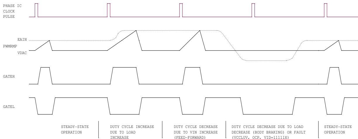
Figure 5 PWM Operating Waveforms
