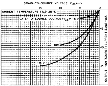
Fig. 10 - Minimum output high (source) current characteristics.
