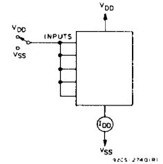
Fig. 17 - Quiescent device current test circuit.
