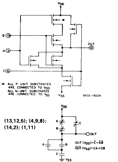
Fig. 2 — Sample COS/MOS logic circuit arrangements using type CD4007UB.
