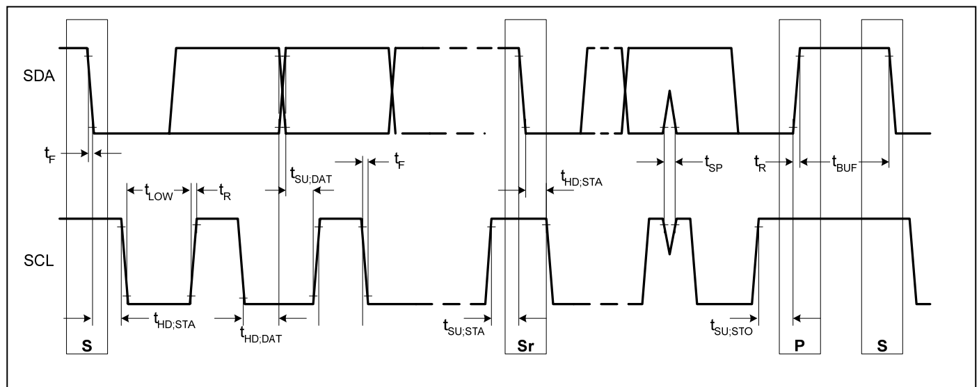
Figure 1. Timing Diagram
