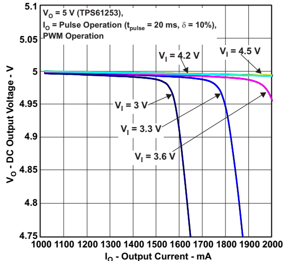
Figure 10. DC Output Voltage vs Output Current
