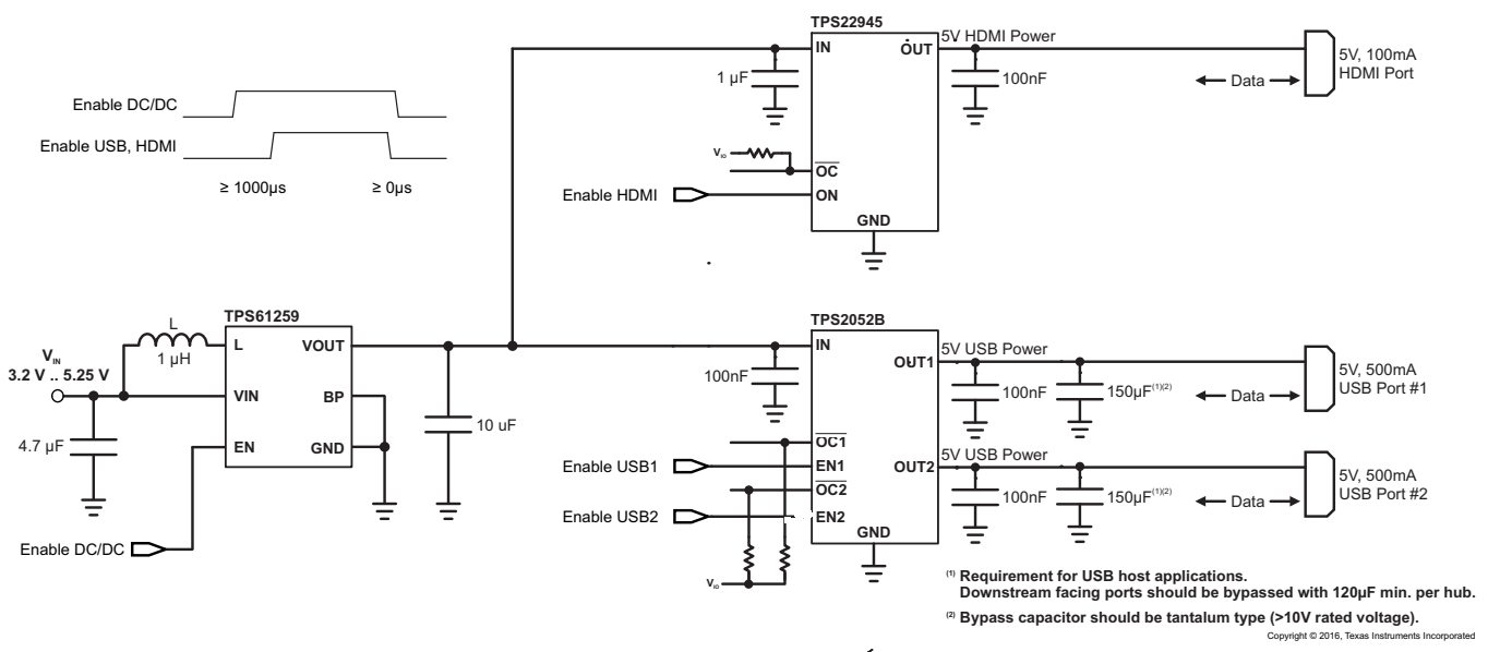
Figure 42. Single Cell Li-Ion Power Solution for Tablet PCs Featuring x2 USB Host Ports, HDMI I/F
