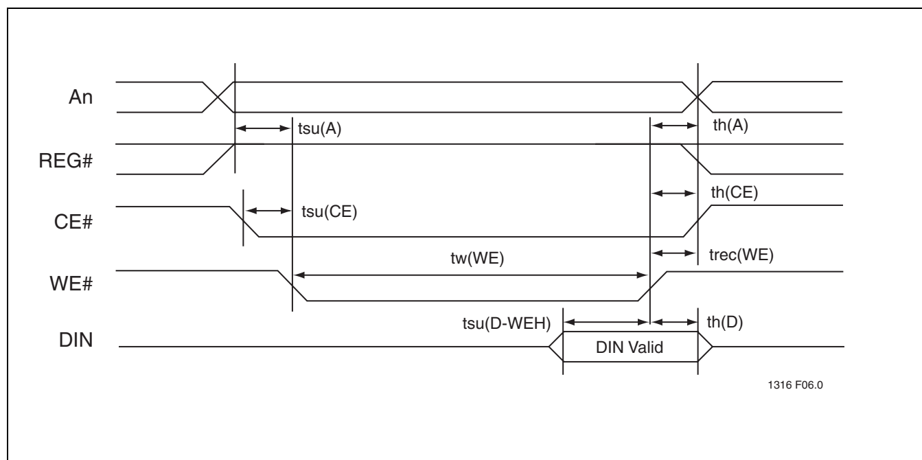
FIGURE 10-5: Common Memory Write Timing Diagram
