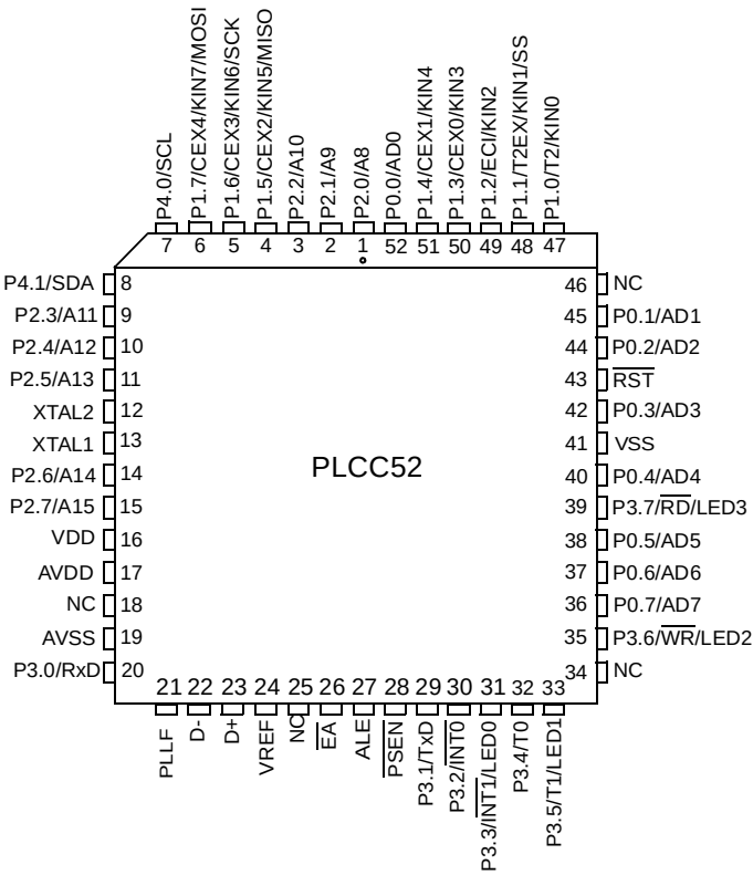
Figure 1. AT89C5131A-L 52-pin PLCC Pinout
