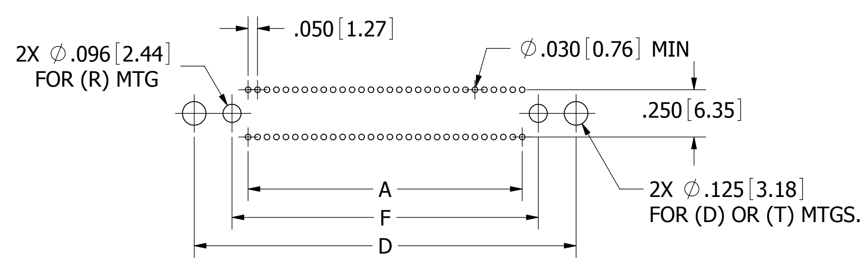
PCB LAYOUT, CONNECTOR SIDE
