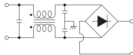
(d) X-capacitor, Y-capacitor, and common mode choke coil all used
