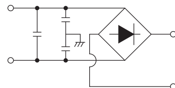
(c) Both X and Y-capacitor used
