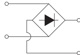
(a) No filter used
