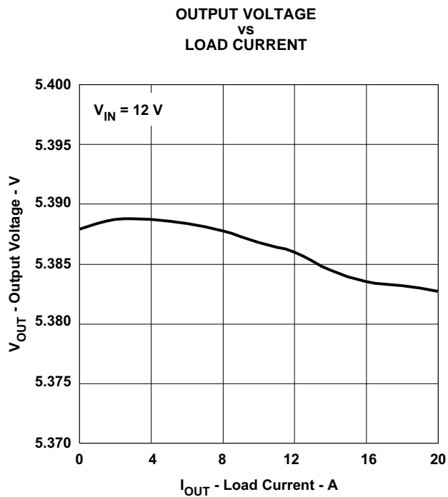
Figure 16. Load Regulation
