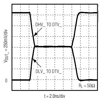
DRIVE TO TERM TRANSITION
