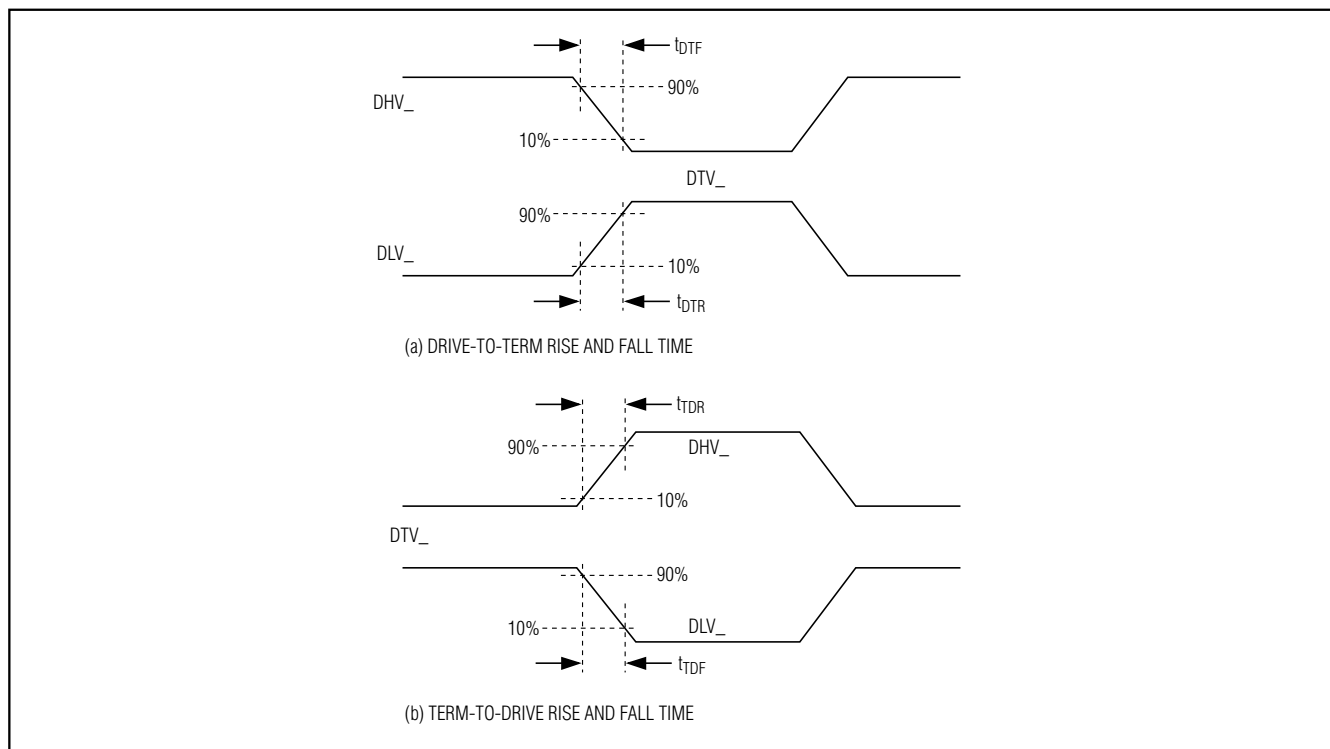
Figure 1. Drive-to-Term and Term-to-Drive Rise and Fall Times
