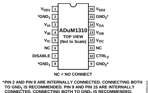
Figure 4. ADuM1310 Pin Configuration
