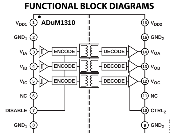
Figure 1. ADuM1310
